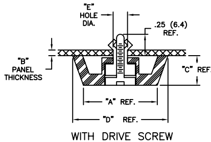
WITH DRIVE SCREW FIGURE 1
