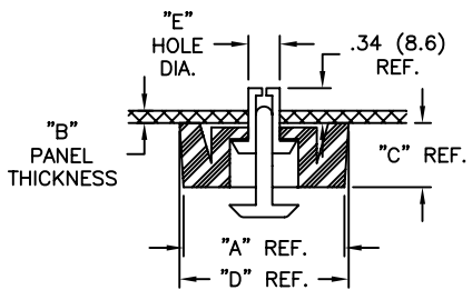
WITH PUSH RIVET FIGURE 2
